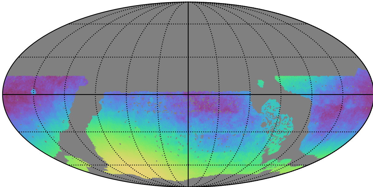
roman_v3.3_10yrs WFD: Normalized Parallax Uncert @ 24.0
