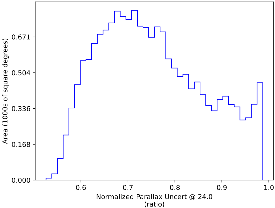
roman_v3.3_10yrs WFD: Normalized Parallax Uncert @ 24.0
