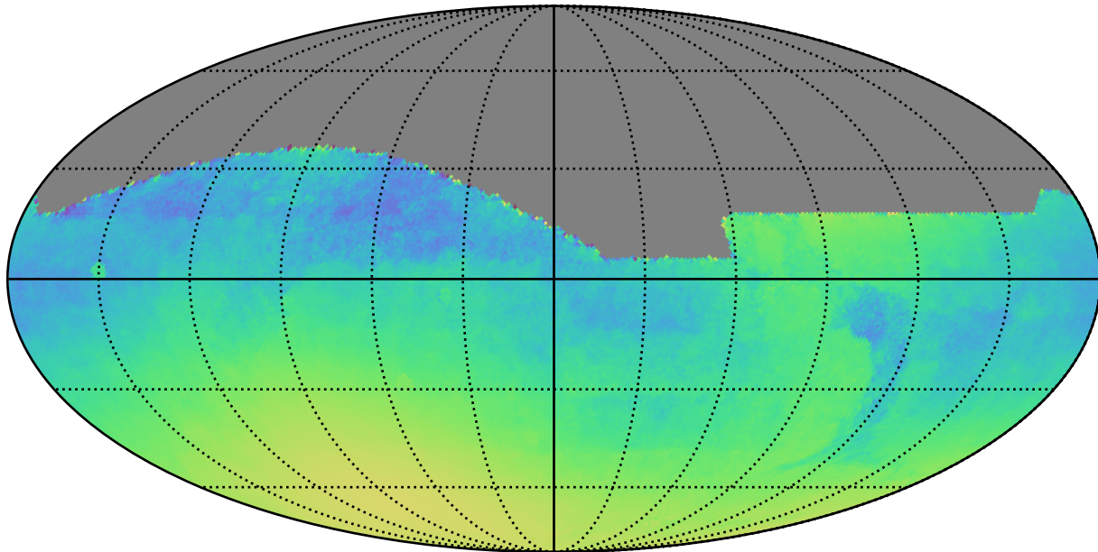
roman_v3.3_10yrs All sky: Normalized Parallax Uncert @ 24.0
