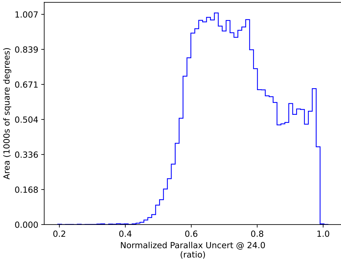
roman_v3.3_10yrs All sky: Normalized Parallax Uncert @ 24.0
