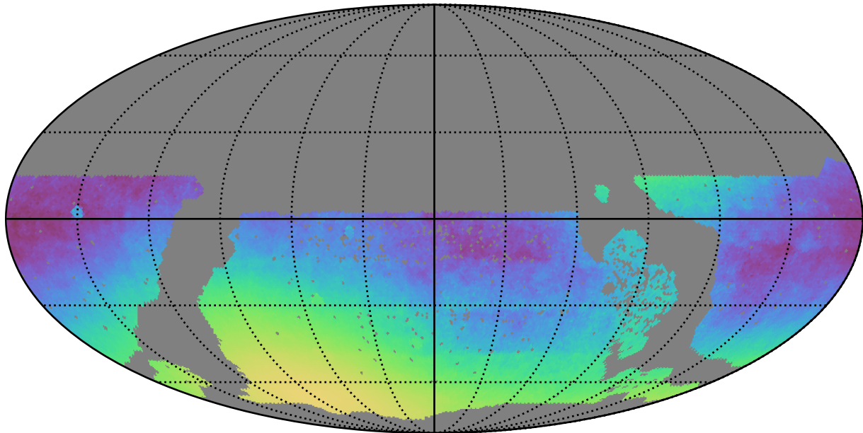
roman_v3.3_10yrs WFD: Normalized Parallax Uncert @ 22.4
