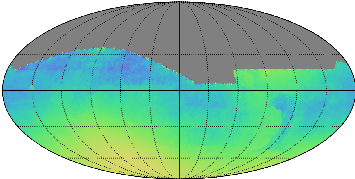
roman_v3.3_10yrs All sky: Normalized Parallax Uncert @ 22.4
