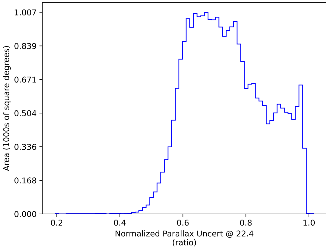
roman_v3.3_10yrs All sky: Normalized Parallax Uncert @ 22.4
