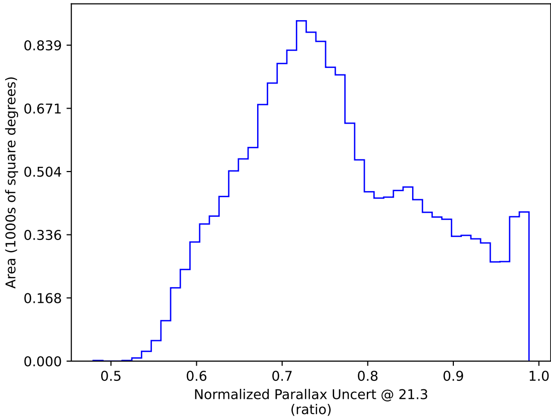
roman_v3.3_10yrs WFD y band only: Normalized Parallax Uncert @ 21.3
