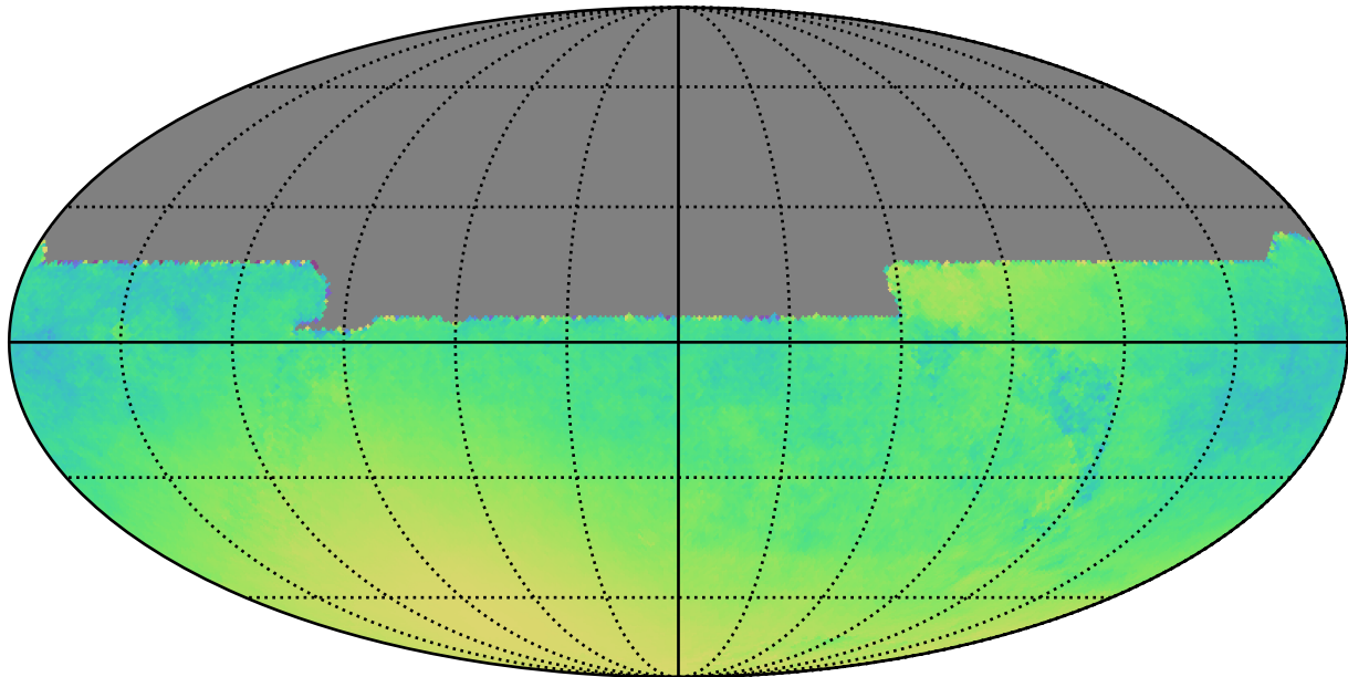
roman_v3.3_10yrs All sky y band only: Normalized Parallax Uncert @ 21.3
