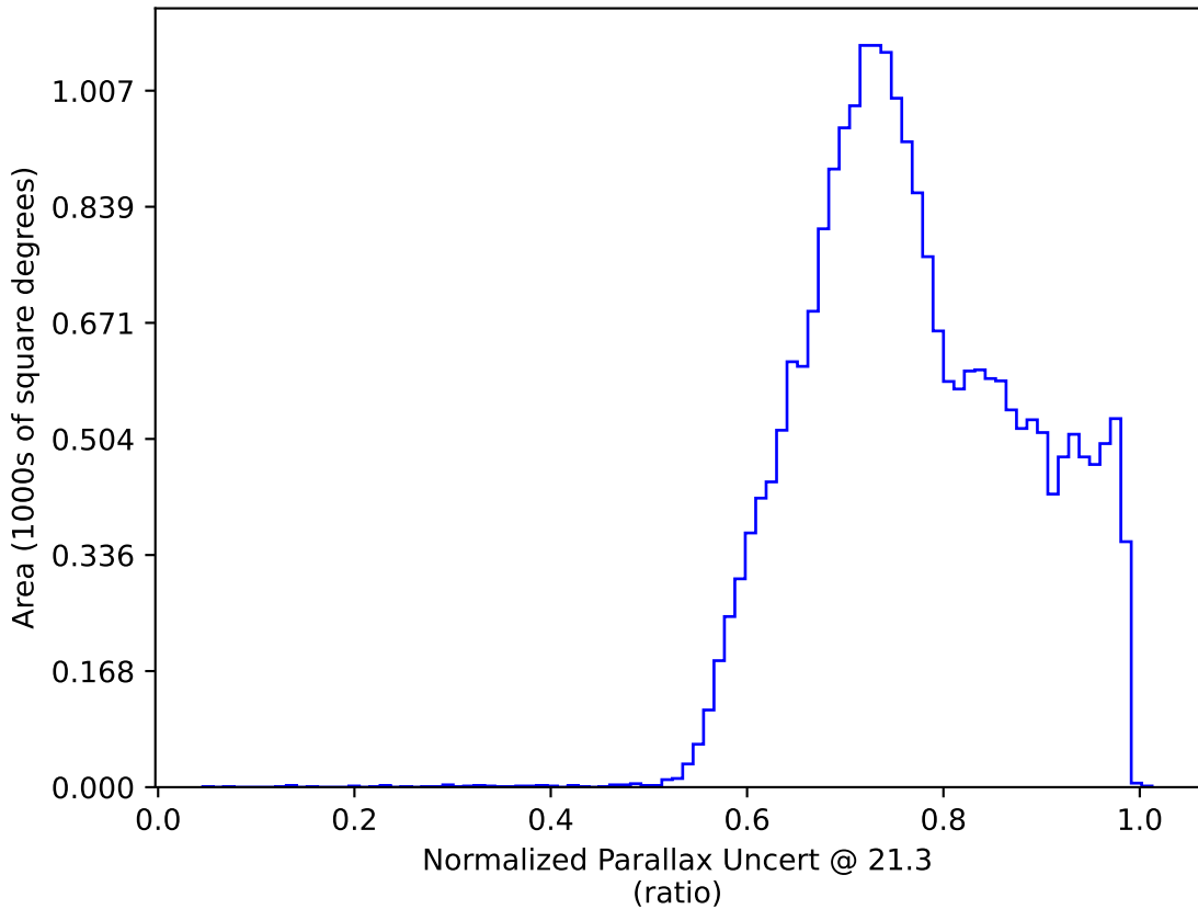
roman_v3.3_10yrs All sky y band only: Normalized Parallax Uncert @ 21.3
