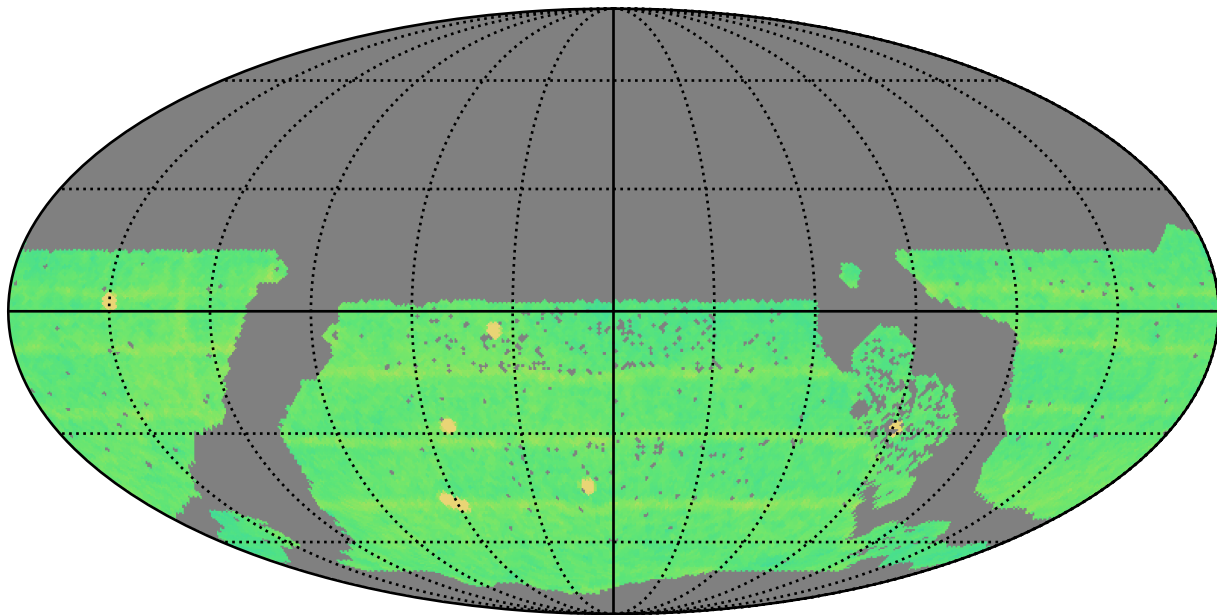
roman_v3.3_10yrs WFD all bands: N Unique Nights
