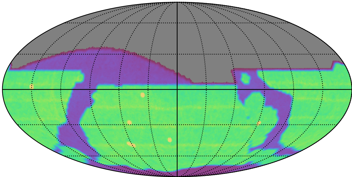
roman_v3.3_10yrs All sky all bands: N Unique Nights
