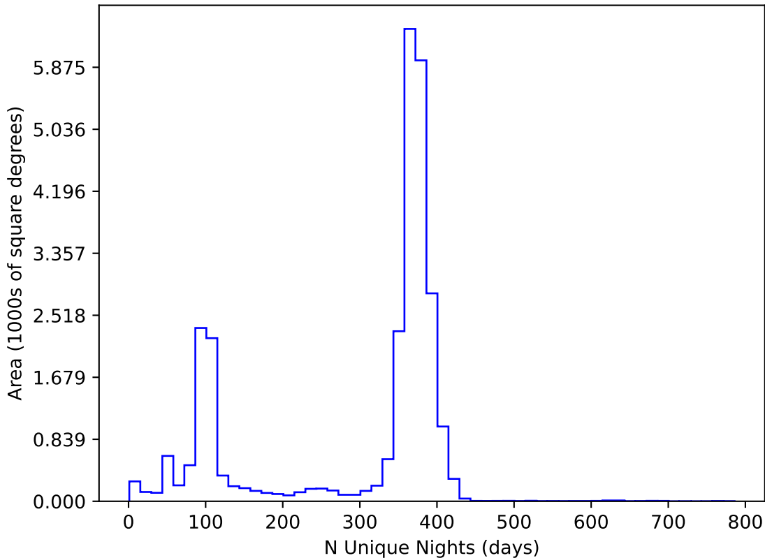
roman_v3.3_10yrs All sky all bands: N Unique Nights
