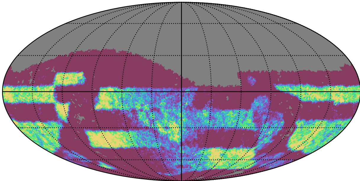
roman_v3.3_10yrs Yr 3-4 z band: NVisits
