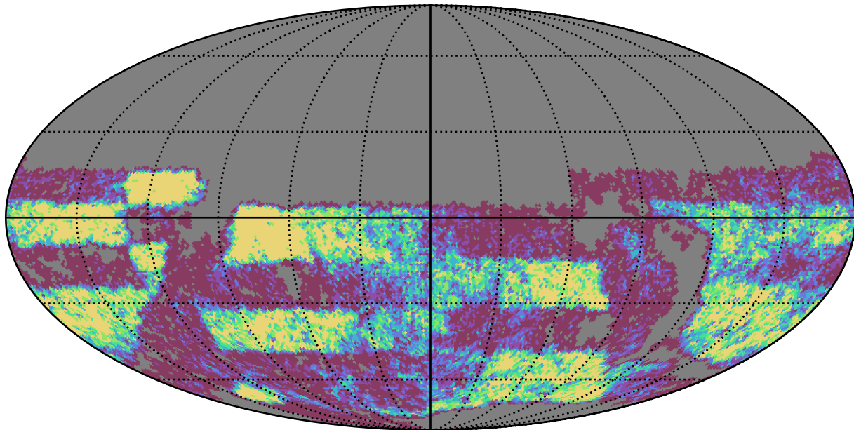
roman_v3.3_10yrs Yr 3-4 u band: NVisits
