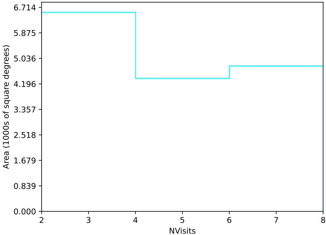
roman_v3.3_10yrs Yr 3-4 u band: NVisits
