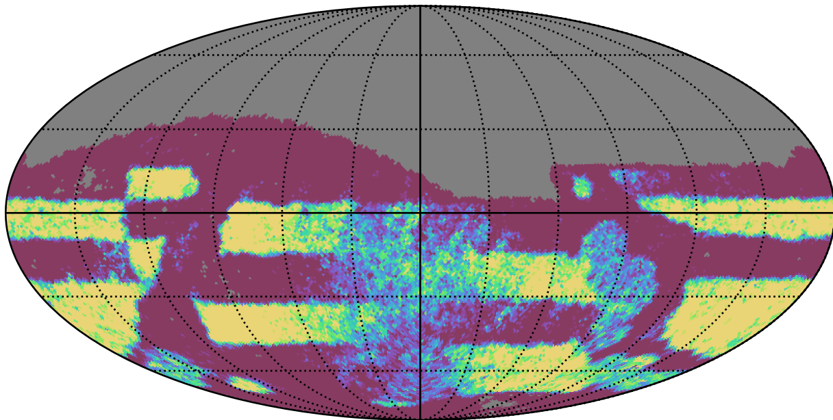
roman_v3.3_10yrs Yr 3-4 r band: NVisits
