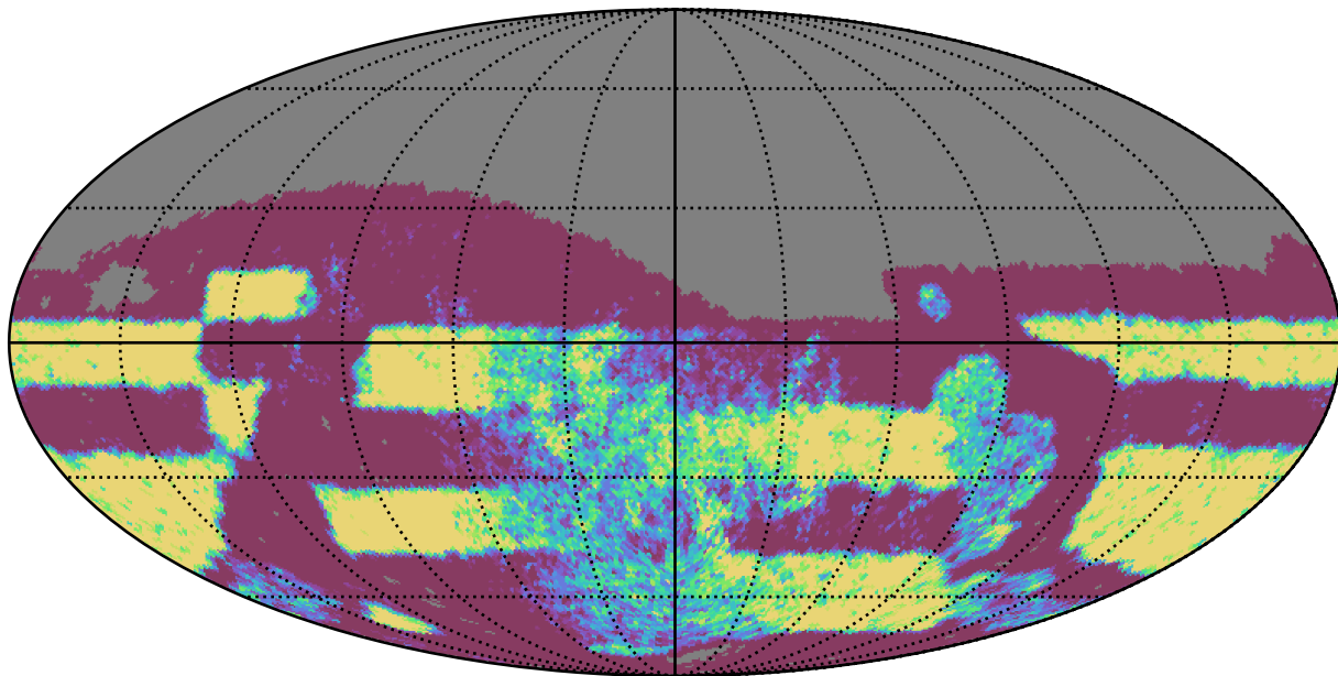
roman_v3.3_10yrs Yr 3-4 i band: NVisits
