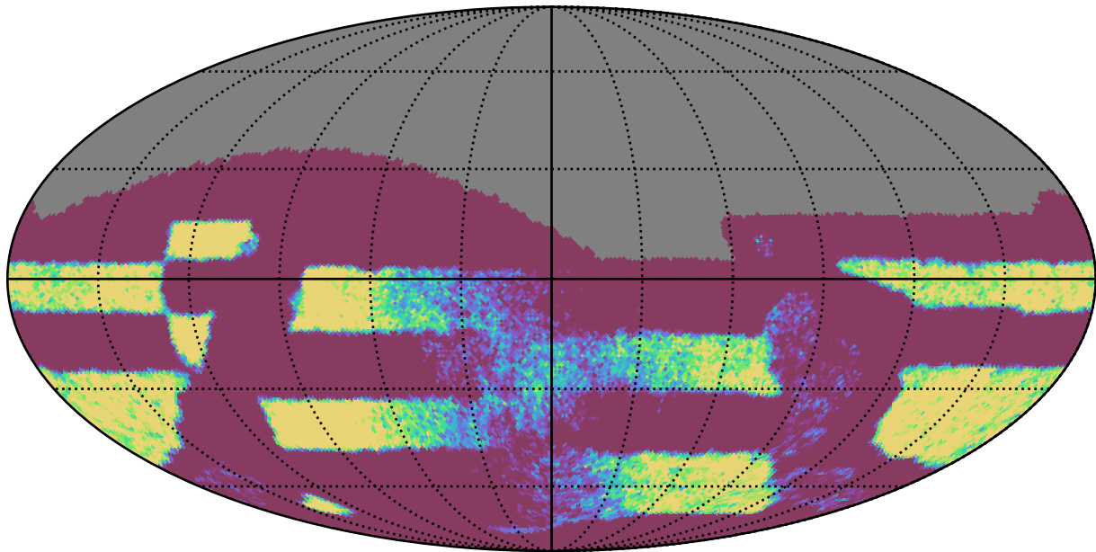
roman_v3.3_10yrs Yr 3-4 all bands: NVisits
