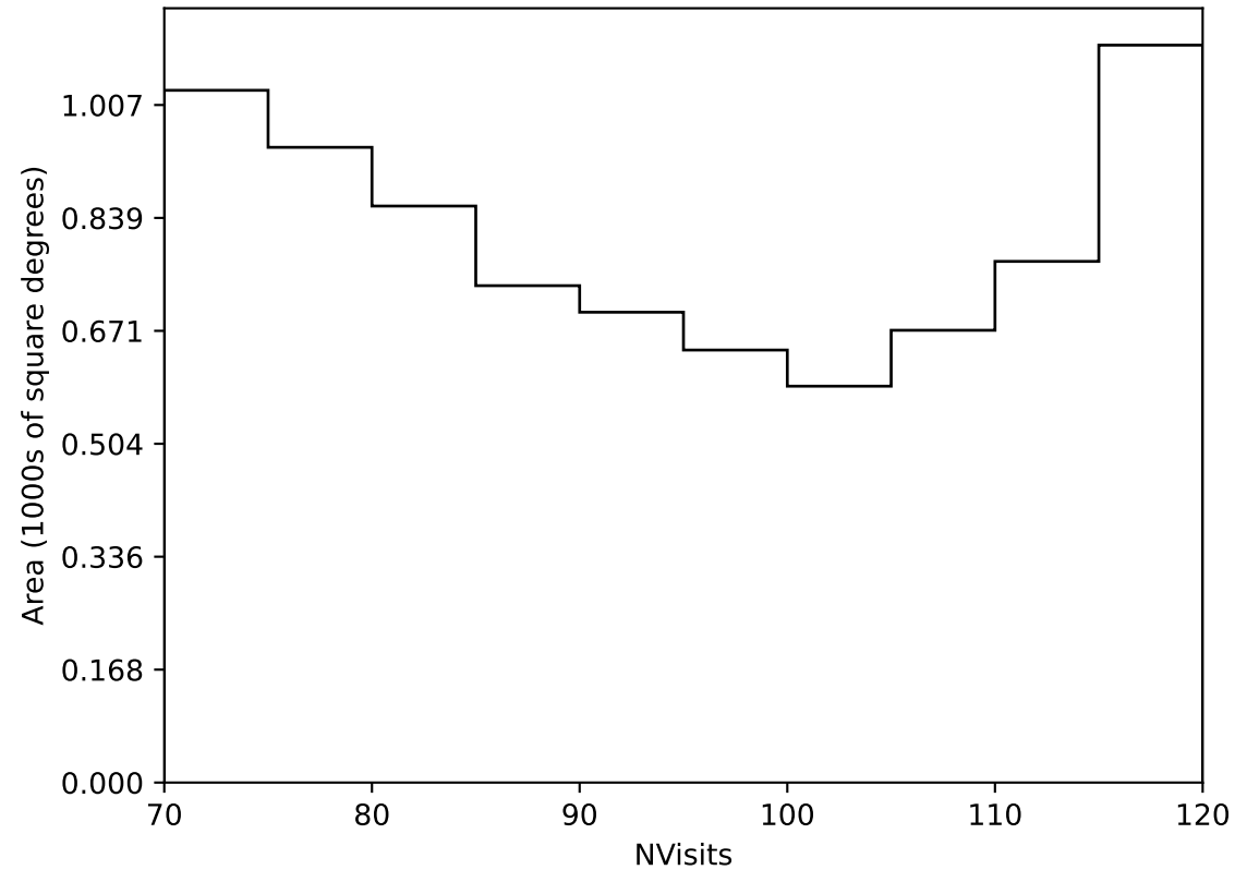
roman_v3.3_10yrs Yr 3-4 all bands: NVisits
