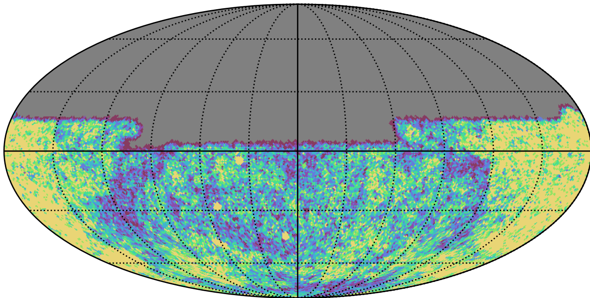
roman_v3.3_10yrs Yr 1 u band: NVisits
