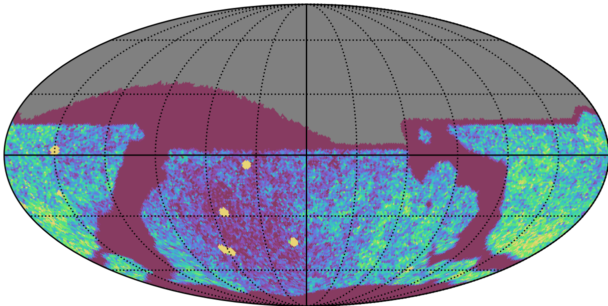
roman_v3.3_10yrs Yr 1 all bands: NVisits
