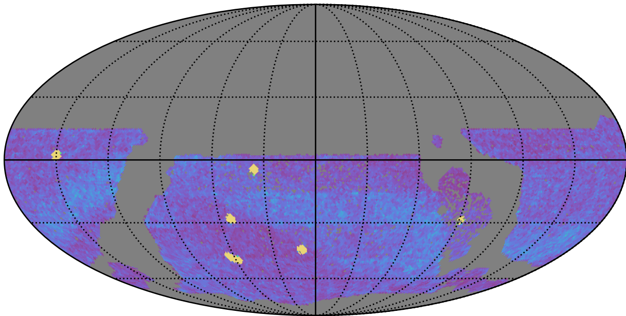
roman_v3.3_10yrs WFD all bands: NVisits
