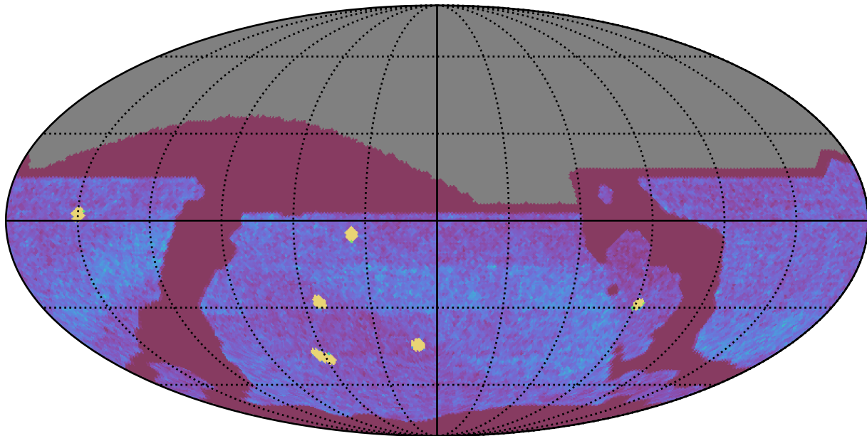
roman_v3.3_10yrs All sky all bands: NVisits
