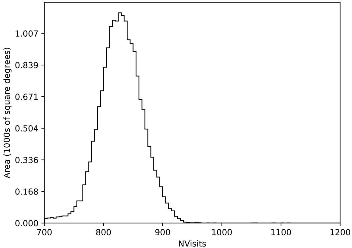
roman_v3.3_10yrs All sky all bands: NVisits
