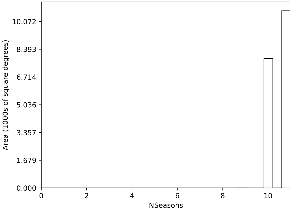
roman_v3.3_10yrs WFD all bands: NSeasons
