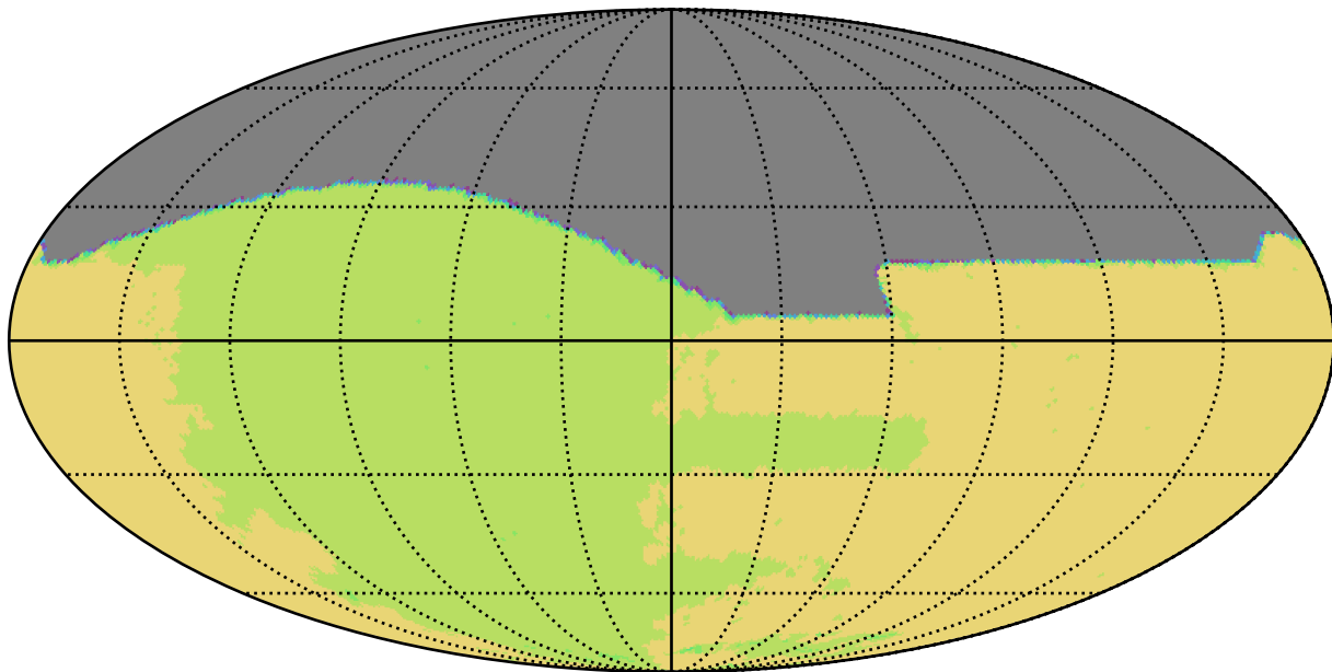
roman_v3.3_10yrs All sky all bands: NSeasons
