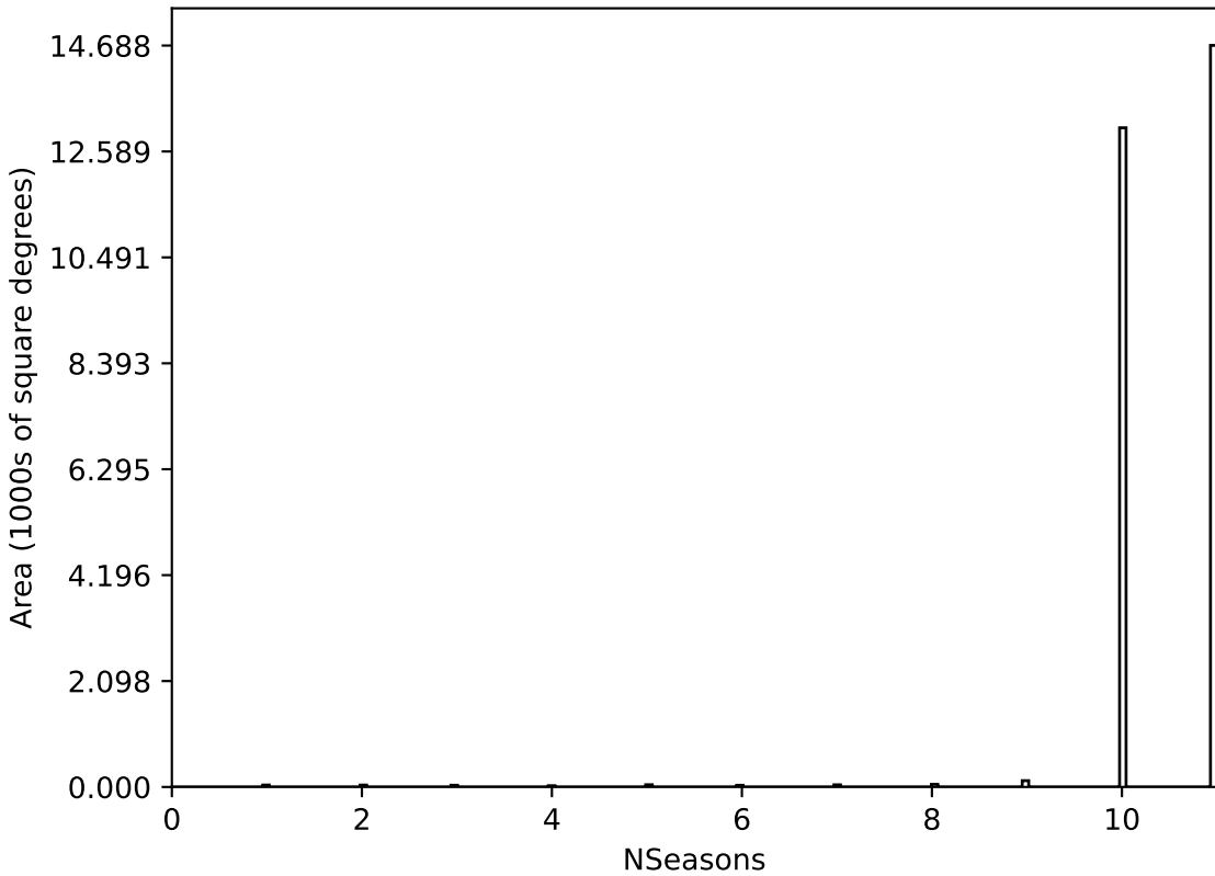
roman_v3.3_10yrs All sky all bands: NSeasons
