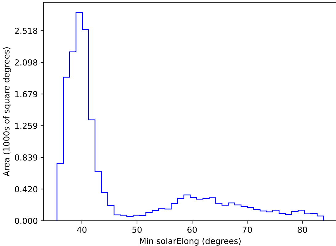
roman_v3.3_10yrs WFD all bands: Min solarElong
