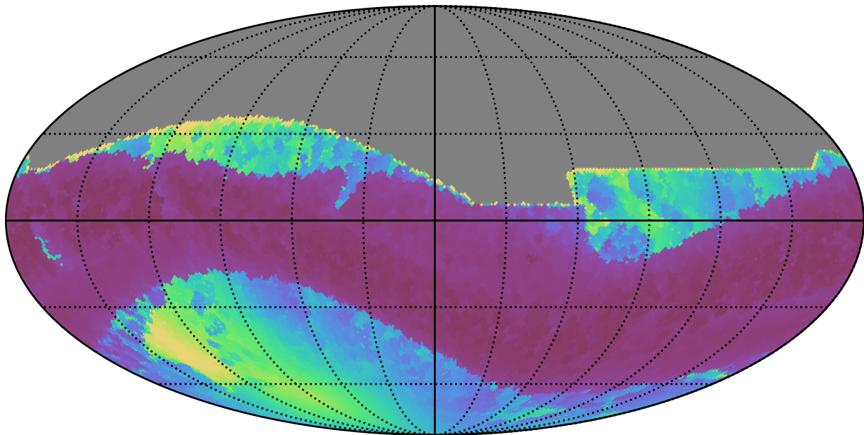
roman_v3.3_10yrs All sky all bands: Min solarElong
