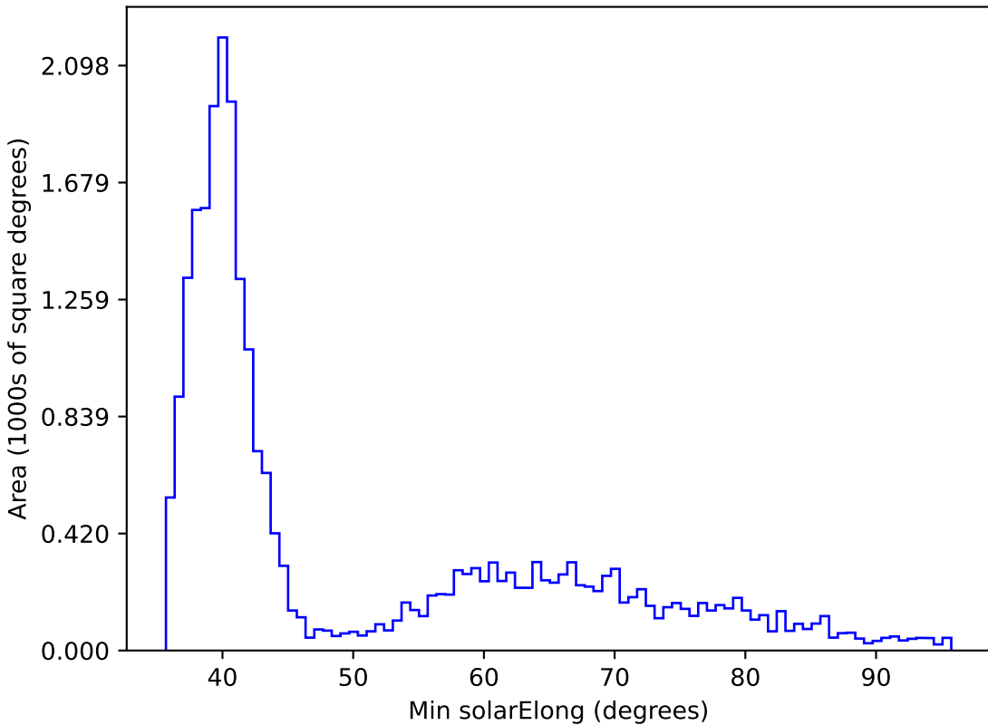
roman_v3.3_10yrs All sky all bands: Min solarElong
