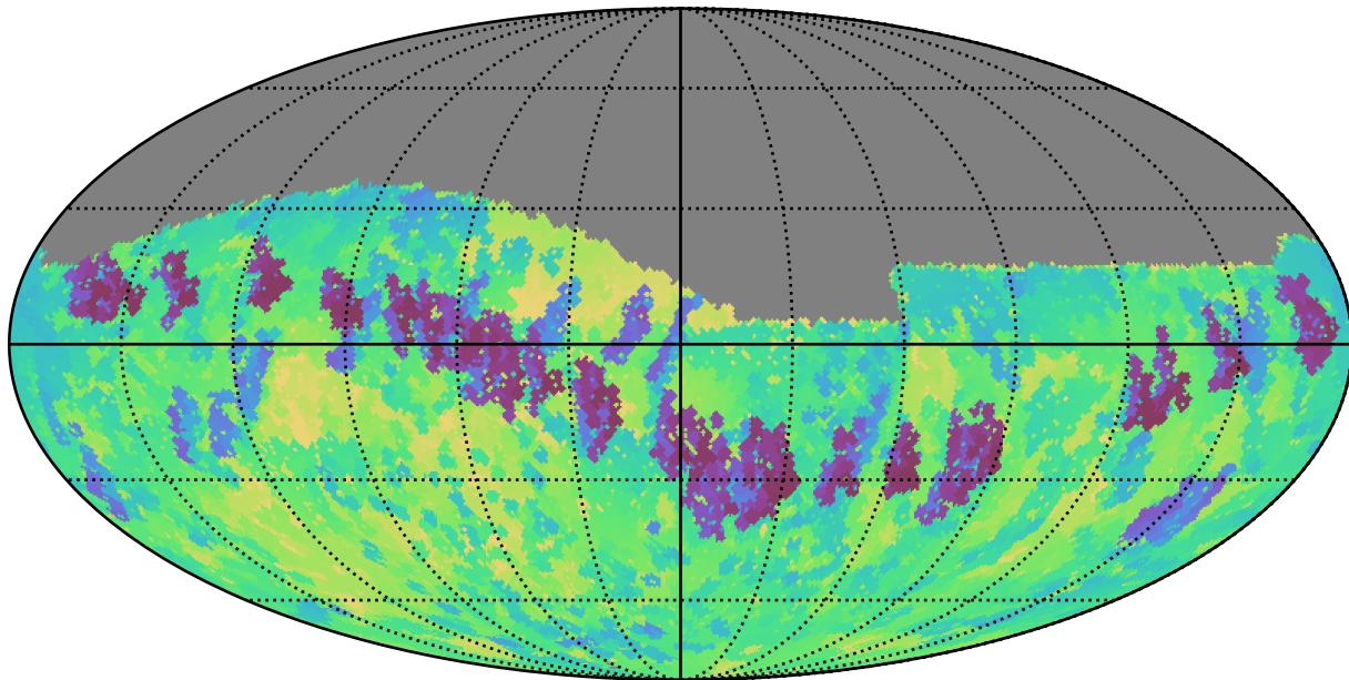
roman_v3.3_10yrs Yr 1 z band: Min skyBrightness
