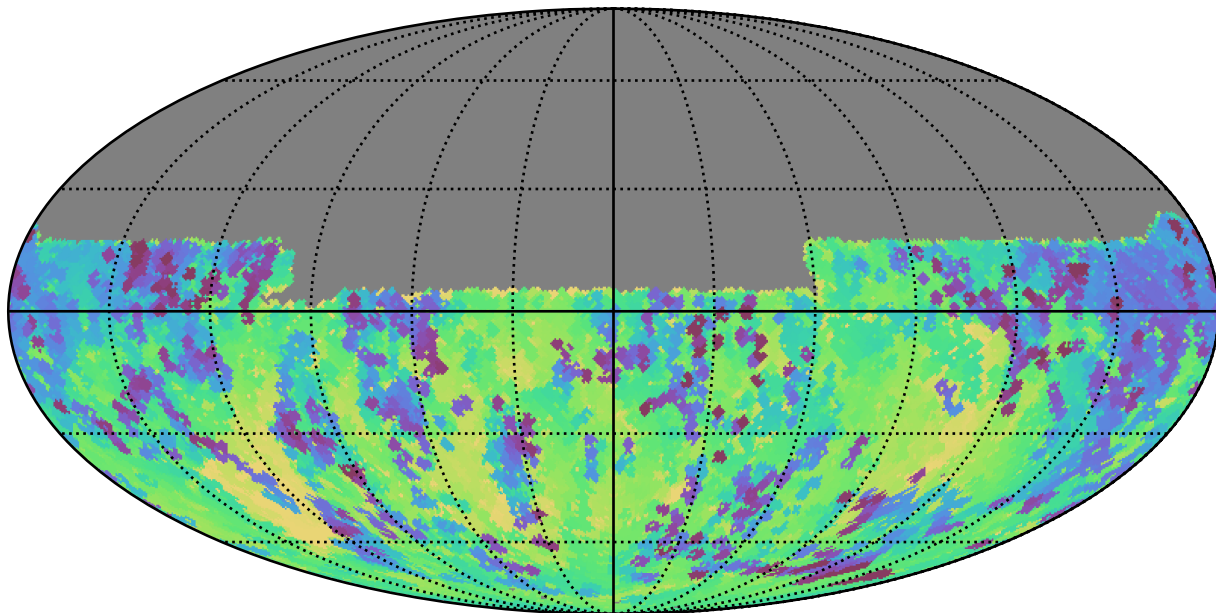
roman_v3.3_10yrs Yr 1 y band: Min skyBrightness
