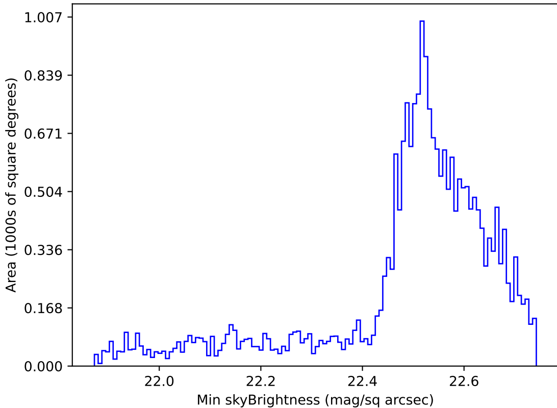
roman_v3.3_10yrs Yr 1 u band: Min skyBrightness
