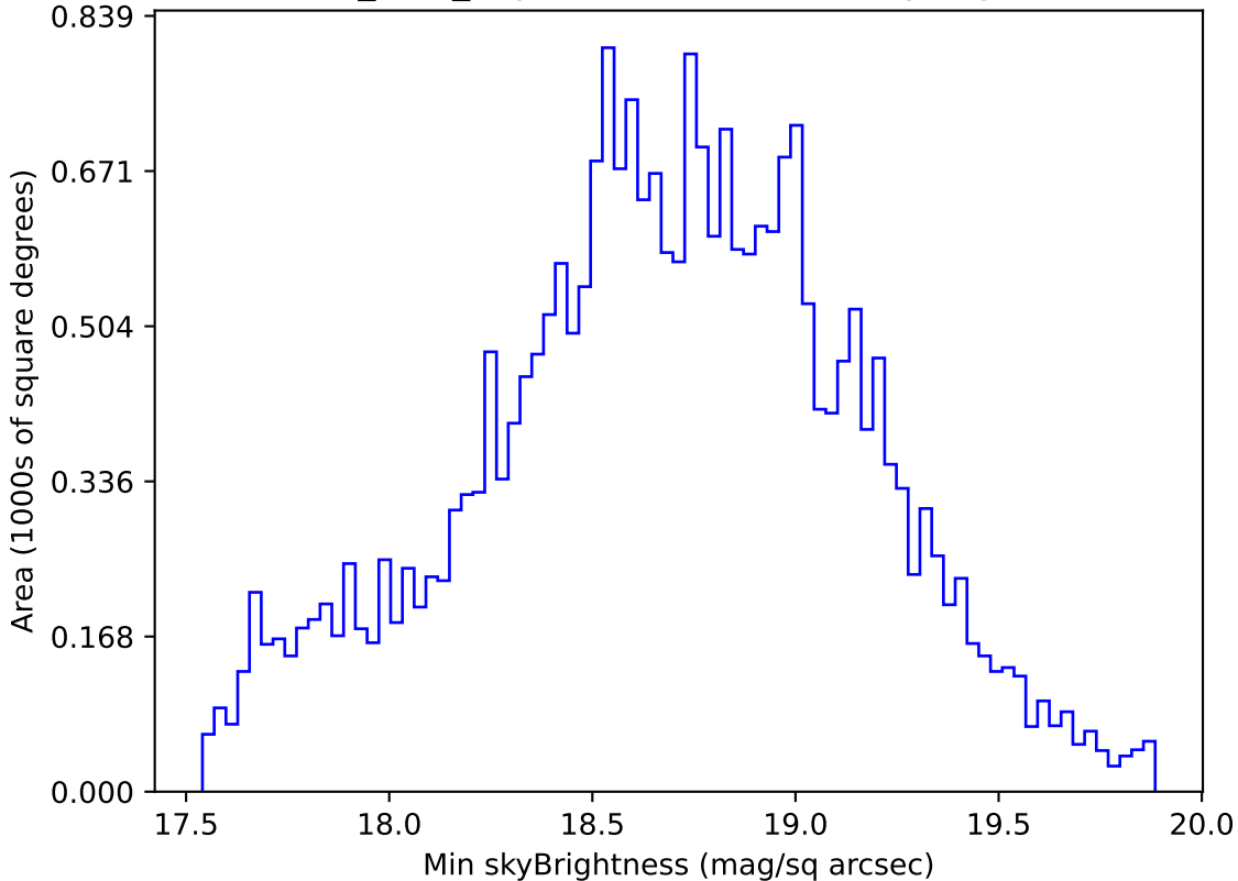
roman_v3.3_10yrs Yr 1 i band: Min skyBrightness
