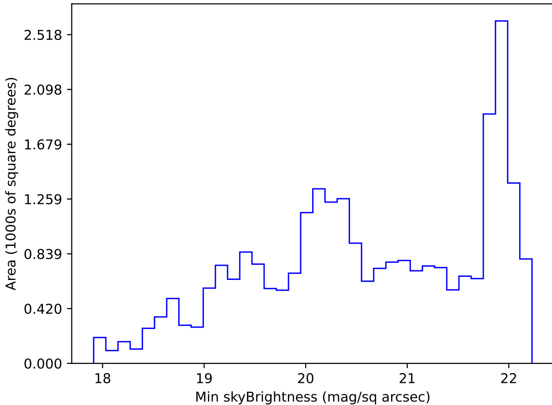
roman_v3.3_10yrs Yr 1 g band: Min skyBrightness
