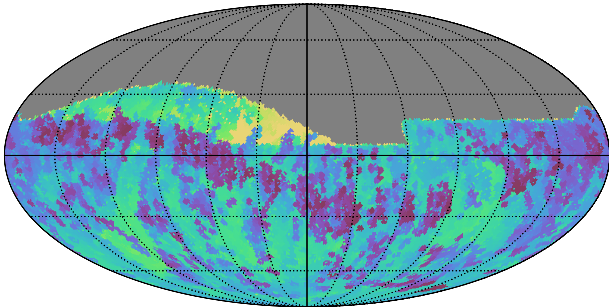
roman_v3.3_10yrs Yr 1 all bands: Min skyBrightness
