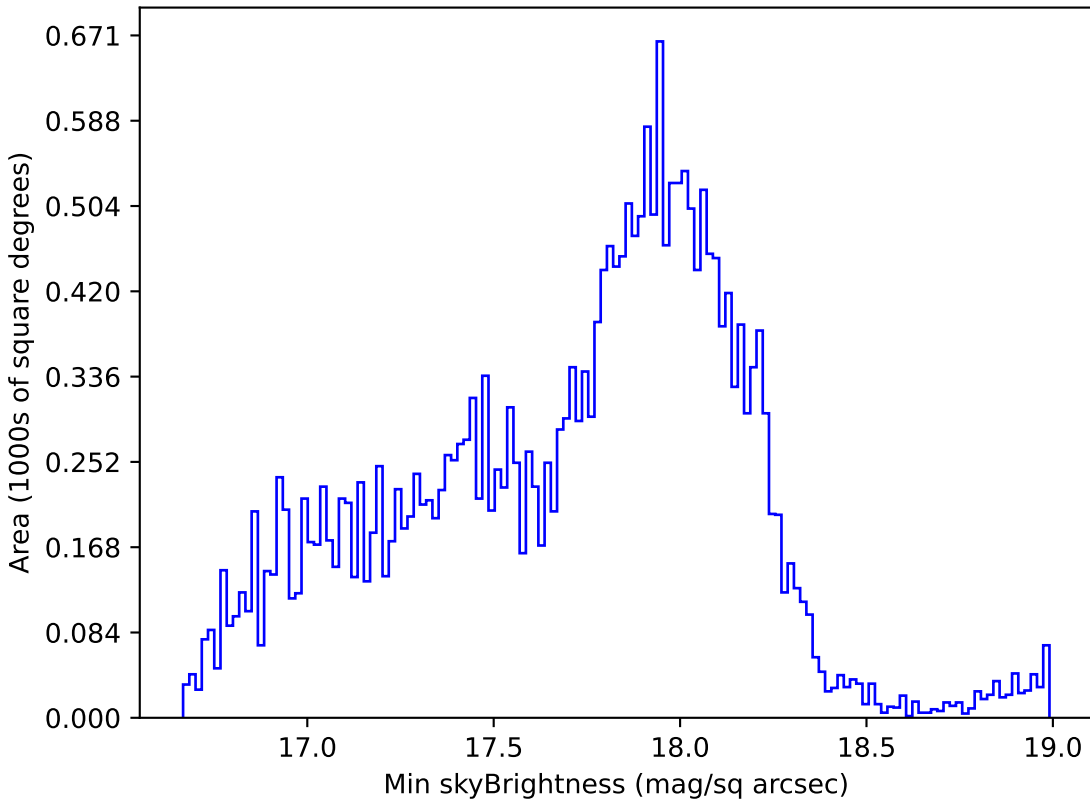
roman_v3.3_10yrs Yr 1 all bands: Min skyBrightness
