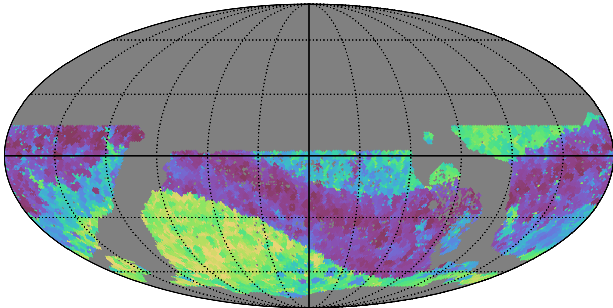
roman_v3.3_10yrs WFD z band: Min skyBrightness
