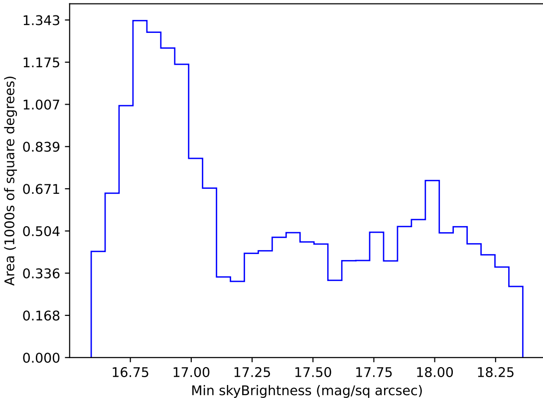
roman_v3.3_10yrs WFD z band: Min skyBrightness
