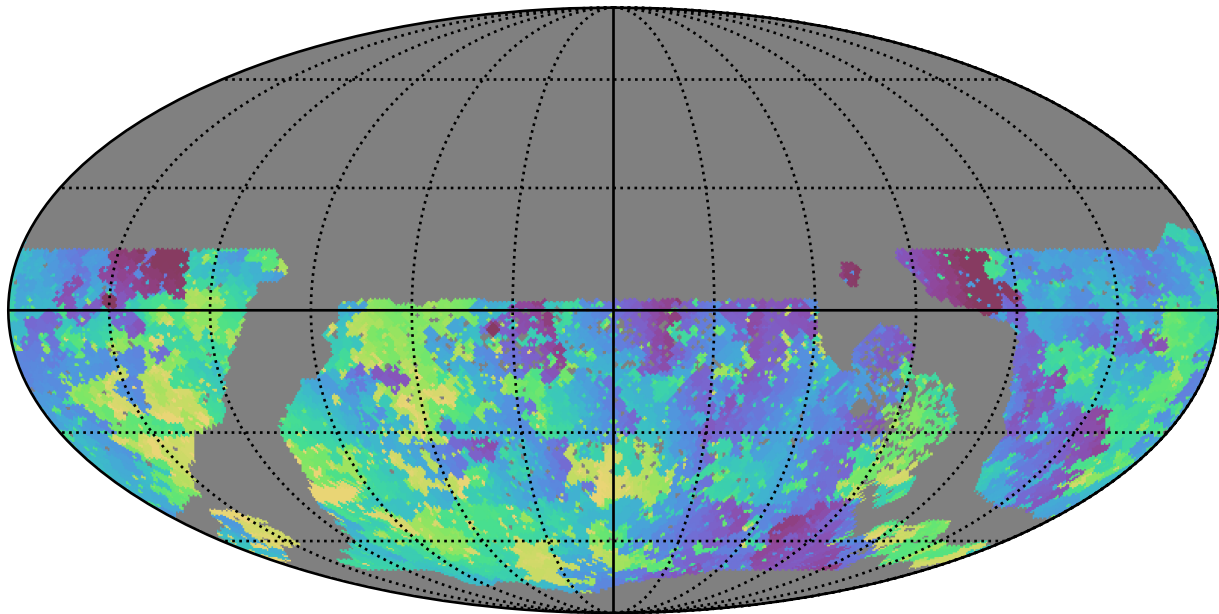
roman_v3.3_10yrs WFD u band: Min skyBrightness
