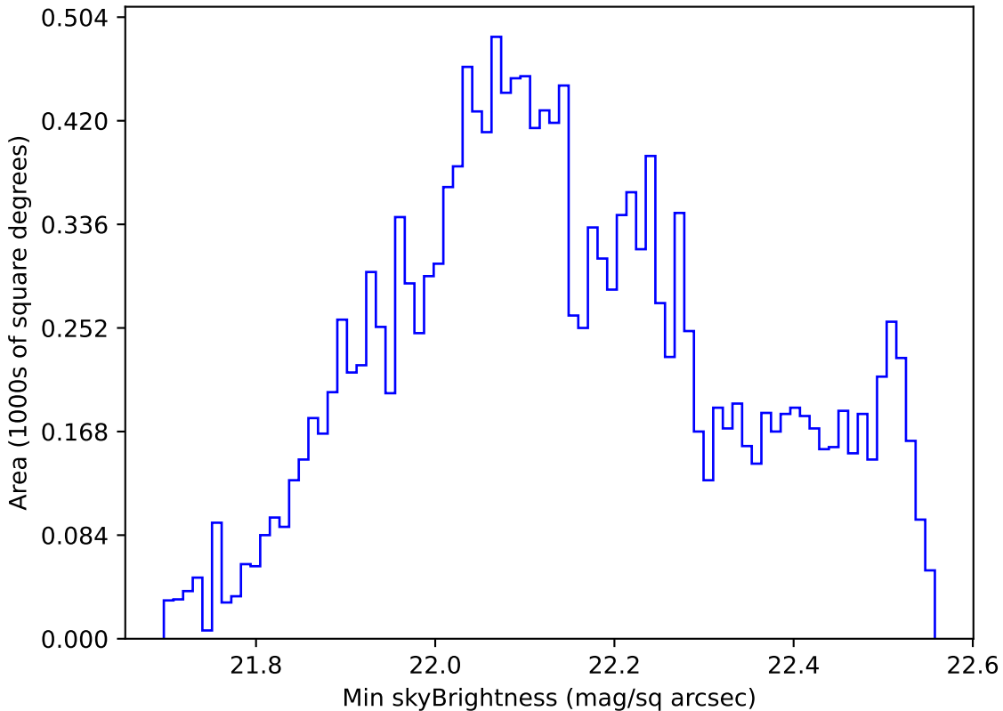
roman_v3.3_10yrs WFD u band: Min skyBrightness
