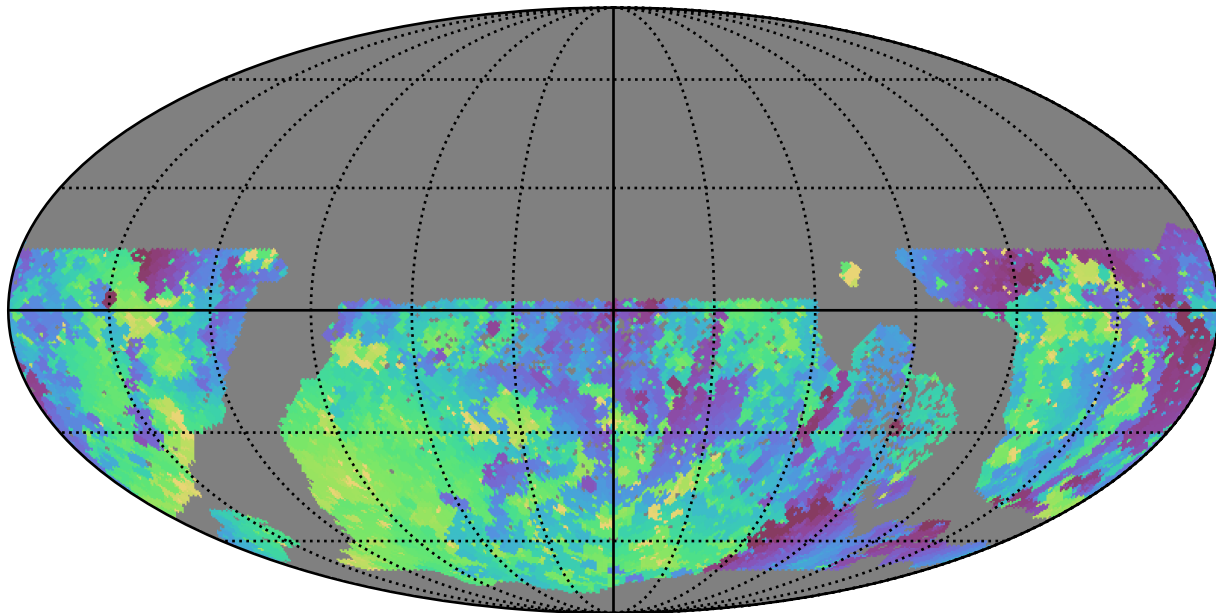
roman_v3.3_10yrs WFD r band: Min skyBrightness
