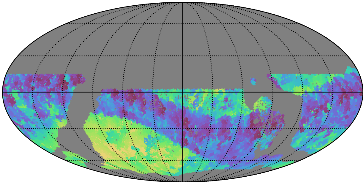
roman_v3.3_10yrs WFD i band: Min skyBrightness
