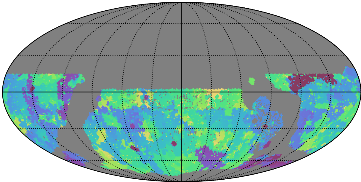
roman_v3.3_10yrs WFD g band: Min skyBrightness
