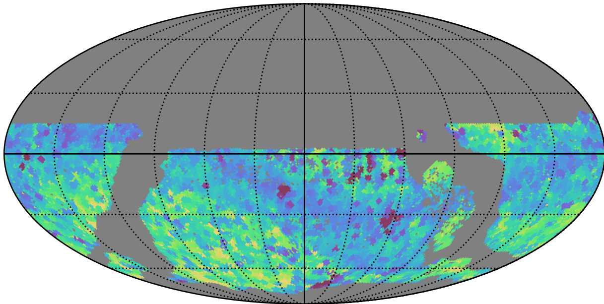
roman_v3.3_10yrs WFD all bands: Min skyBrightness
