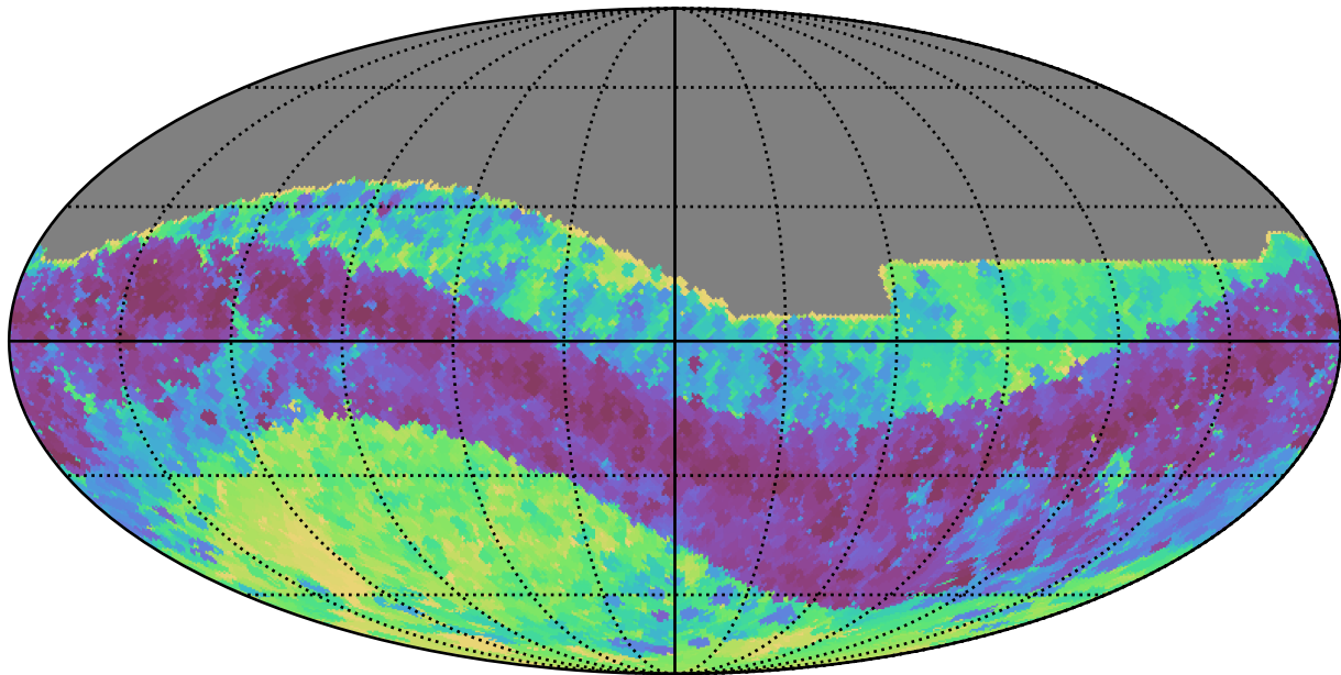
roman_v3.3_10yrs All sky z band: Min skyBrightness
