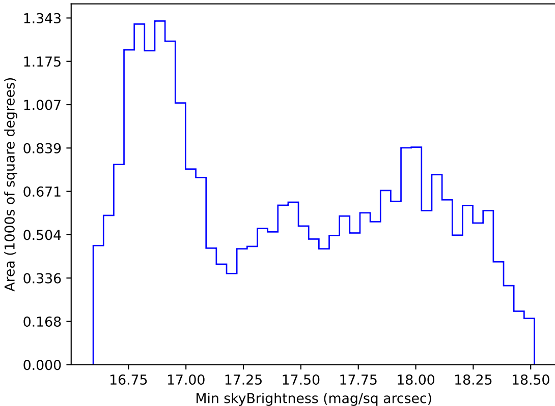
roman_v3.3_10yrs All sky z band: Min skyBrightness
