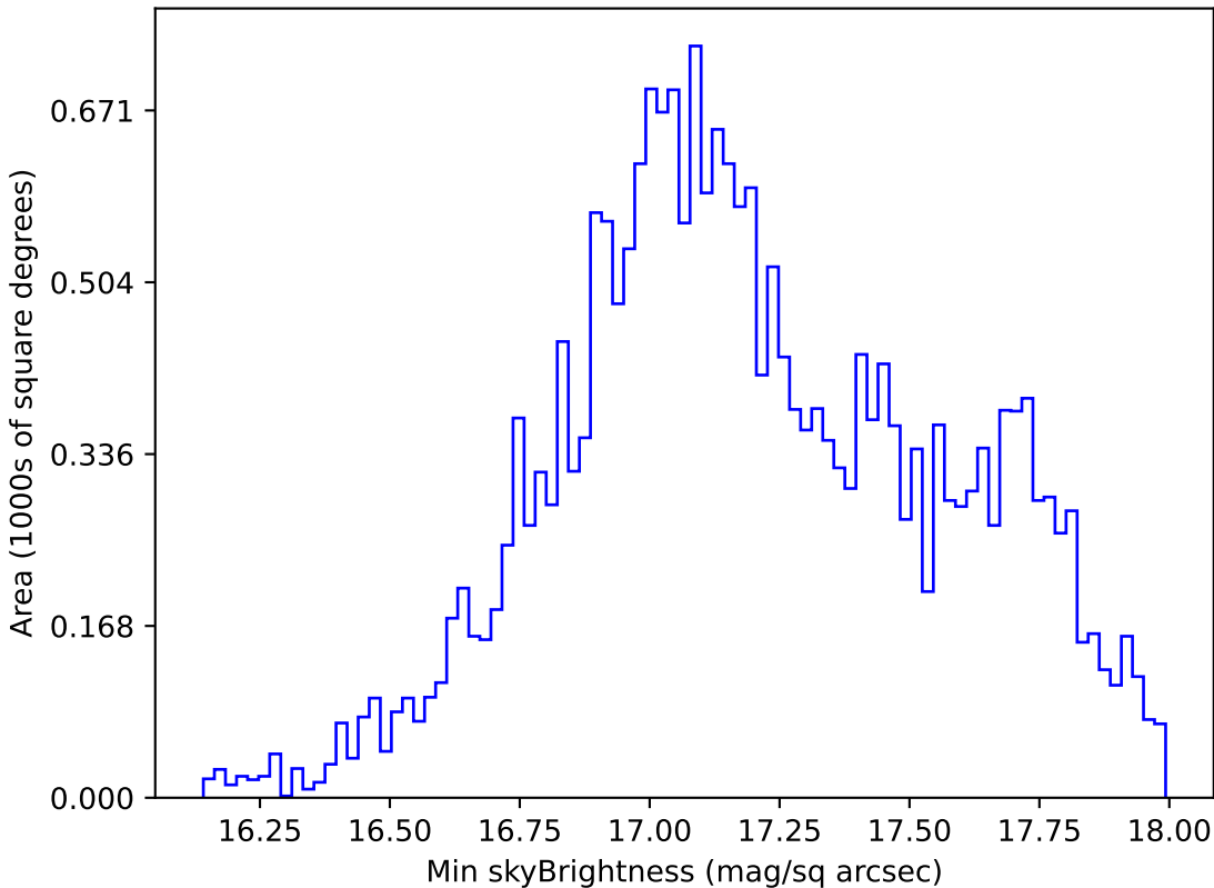
roman_v3.3_10yrs All sky y band: Min skyBrightness
