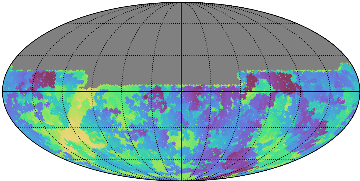
roman_v3.3_10yrs All sky u band: Min skyBrightness
